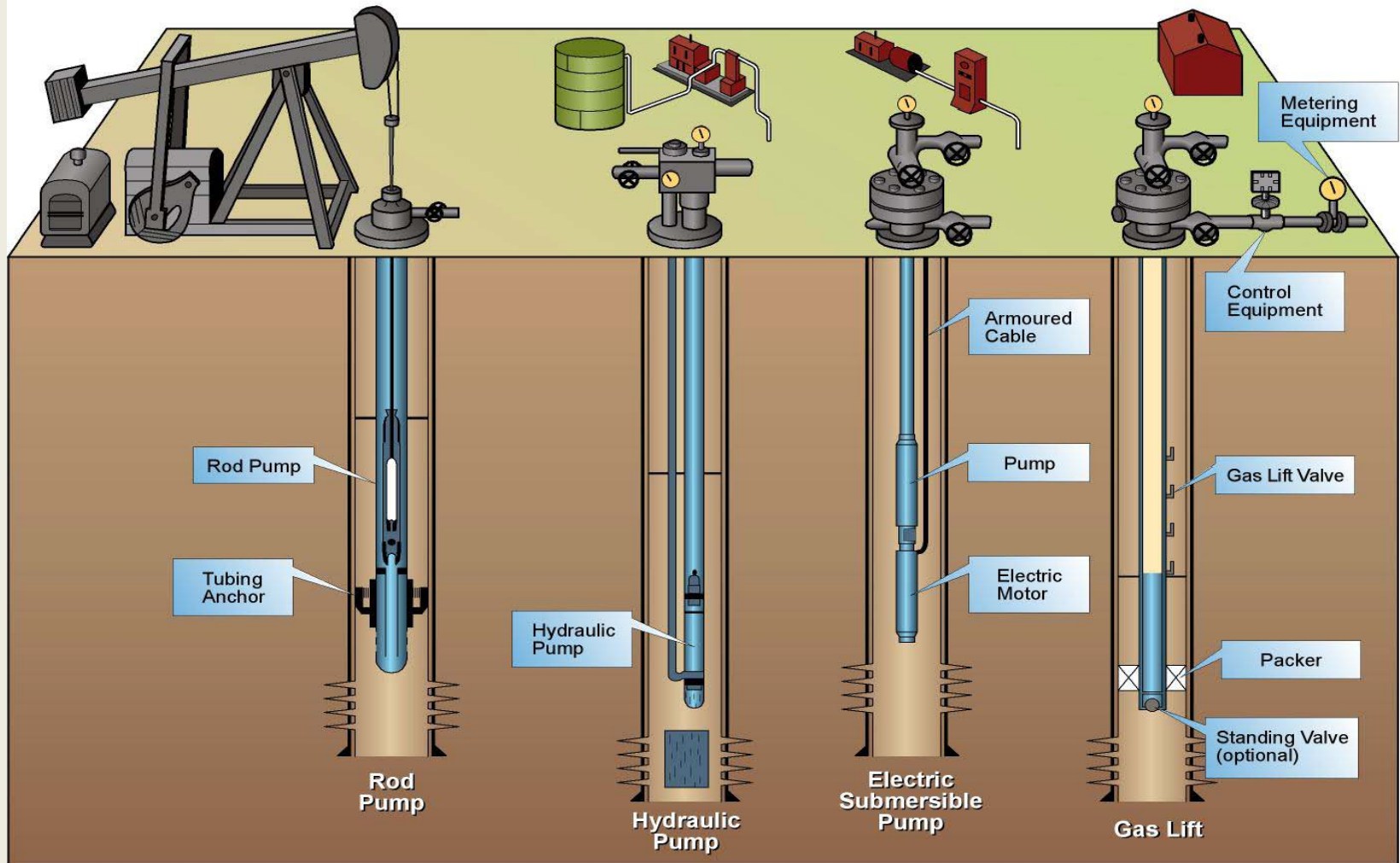
Examples of Artificial Lift Systems
